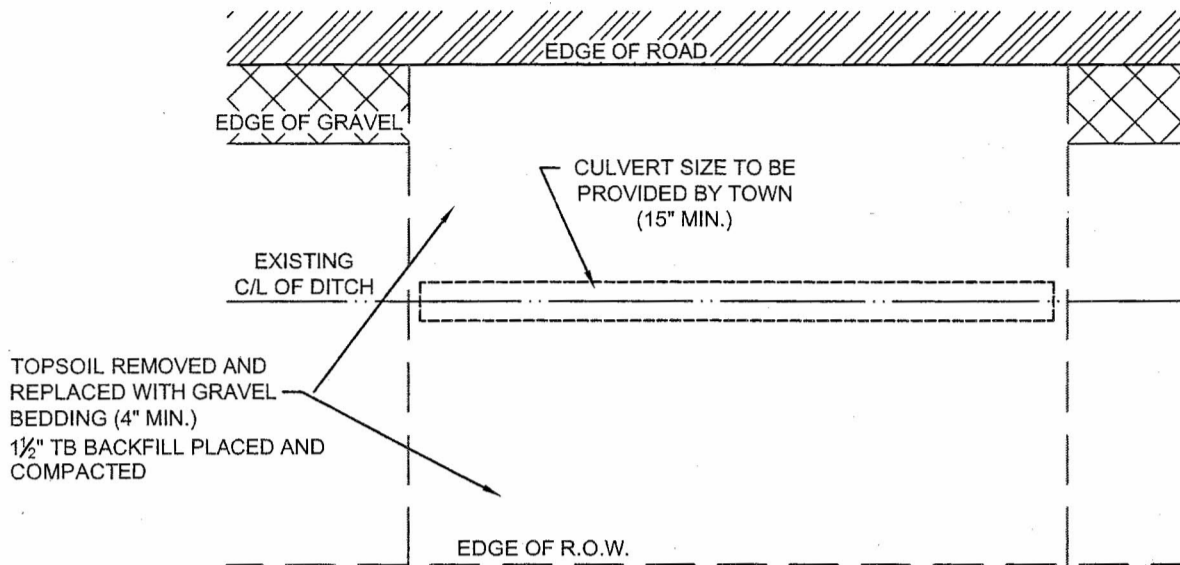
PLAN VIEW
